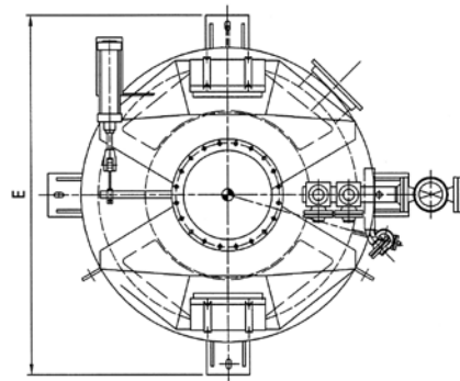
Sketch of typical UNEX™ P economizer. Each economizer is tailor-made to suit the engine data.
